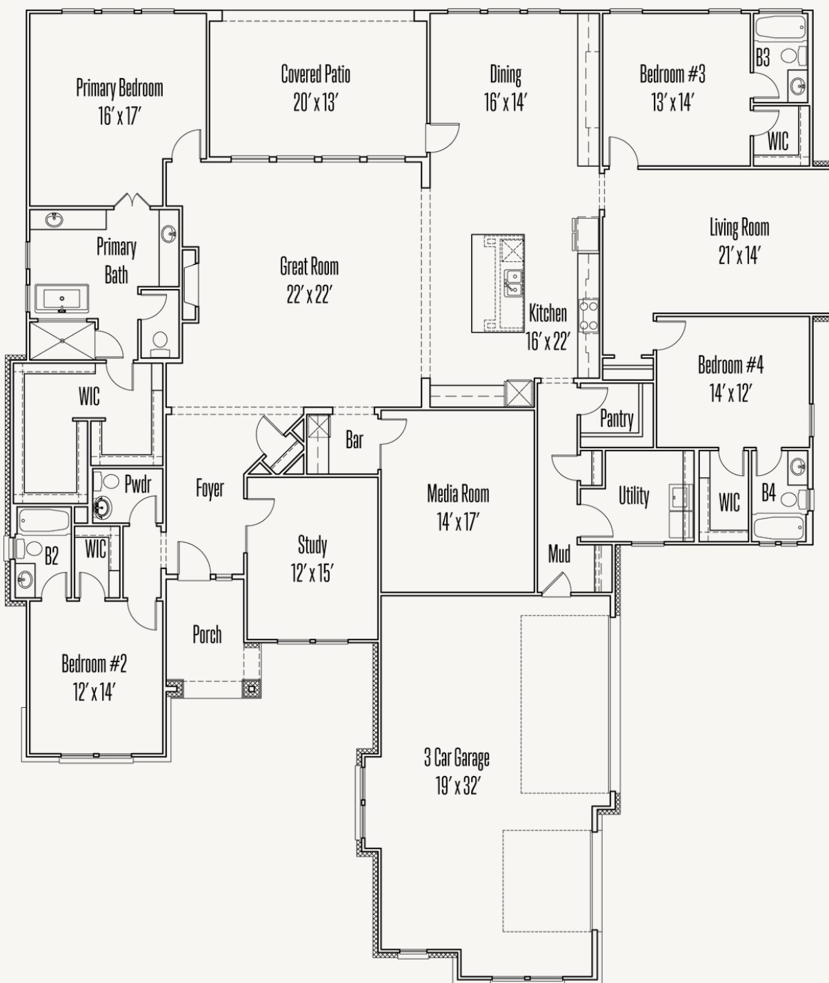
FLOOR PLAN_A
