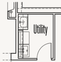
Optional Single Base & Upper Cabinets at Utility
