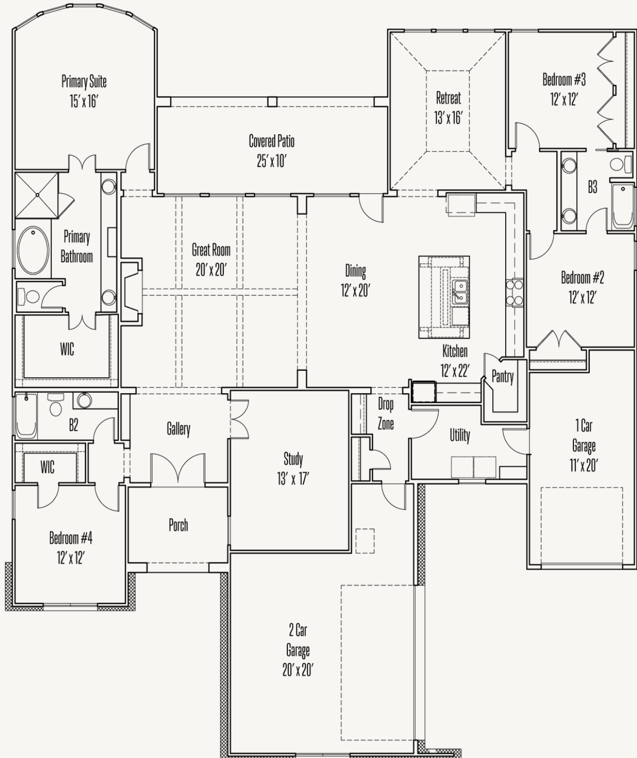
FLOOR PLAN_B
