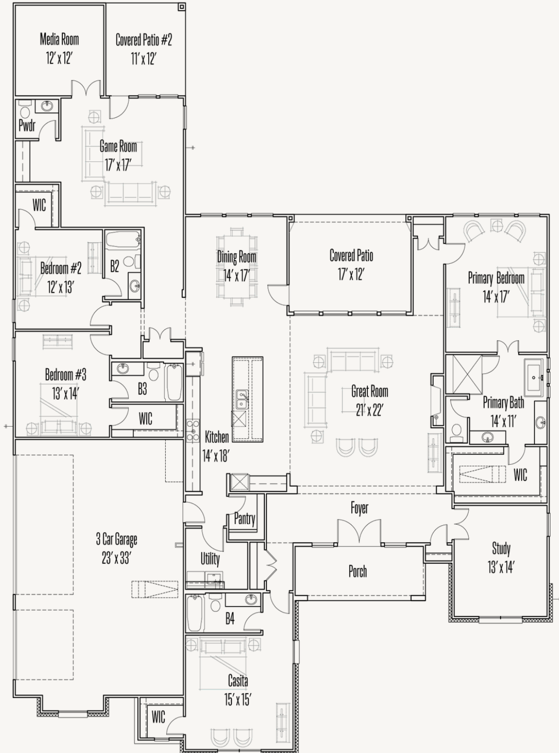
FLOOR PLAN_A
