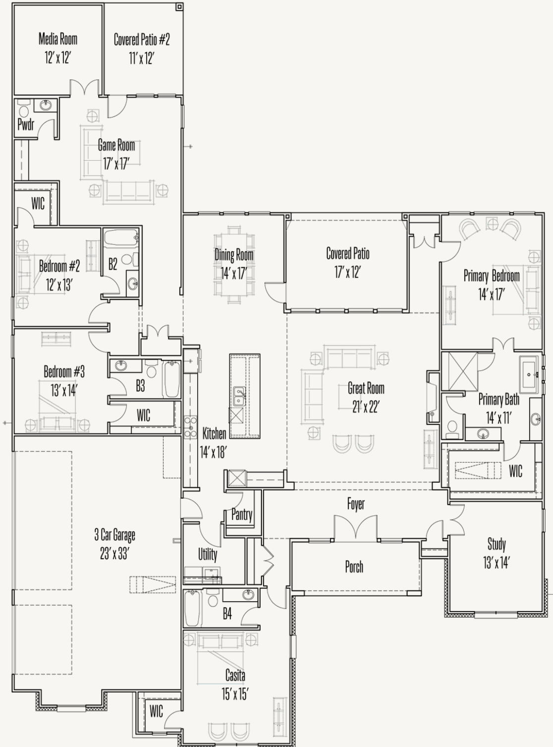
FLOOR PLAN_A
