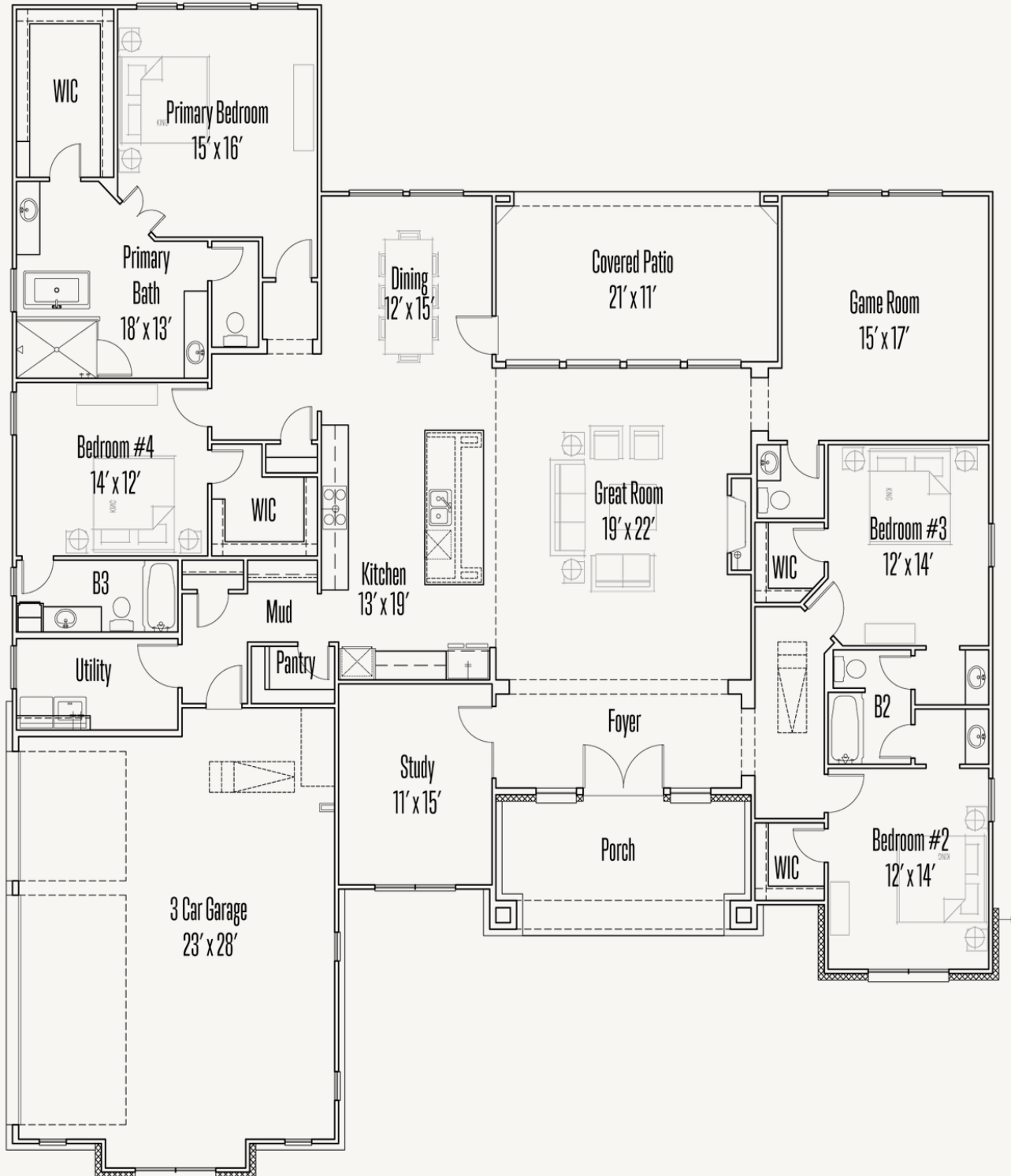
FLOOR PLAN_A
