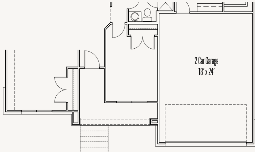
Optional 3'-0" Garage Extension
