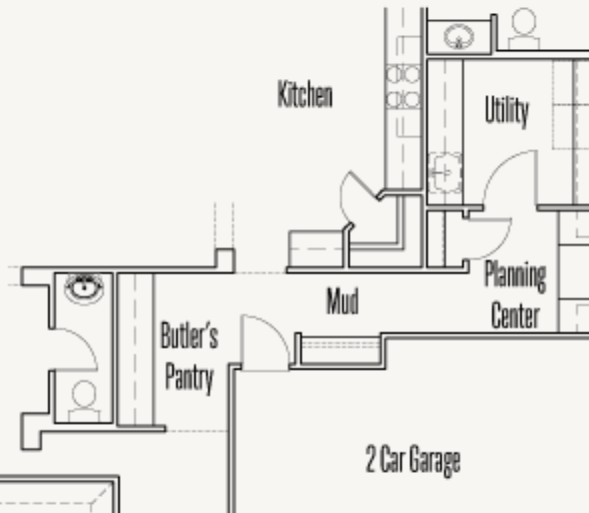
Optional Butler's Pantry, Planning Center and Extended Utility ilo Utility and Tandem Garage
