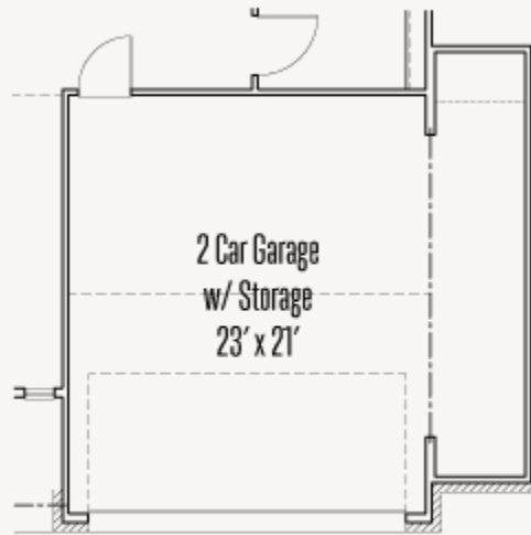
Optional Storage at 2 Car Garage
