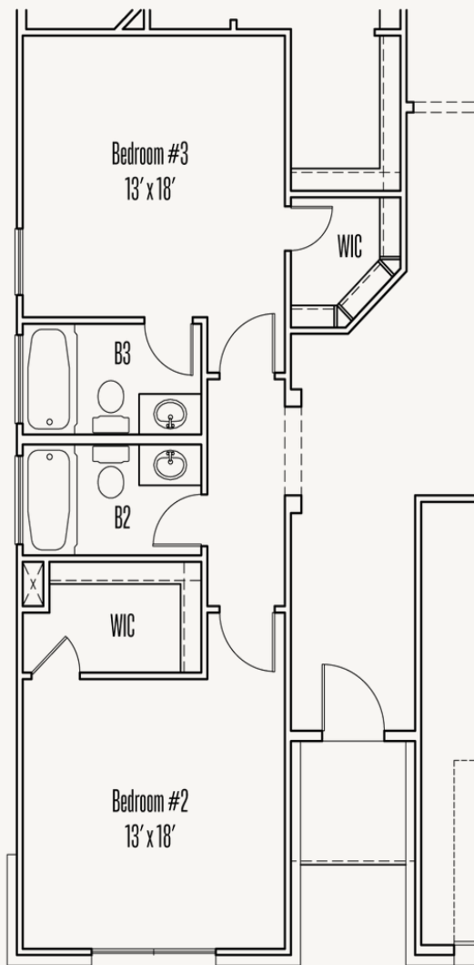
Enlarged Bed #2 & Bed #3 and add Bath #3 ilo Flex Room
