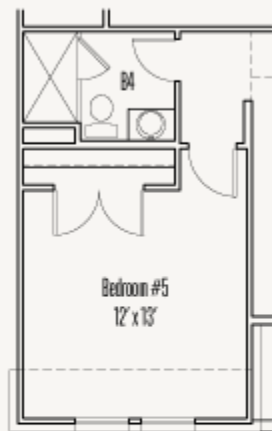
Optional Bedroom #5 and Bath 4 and Study & Powder
