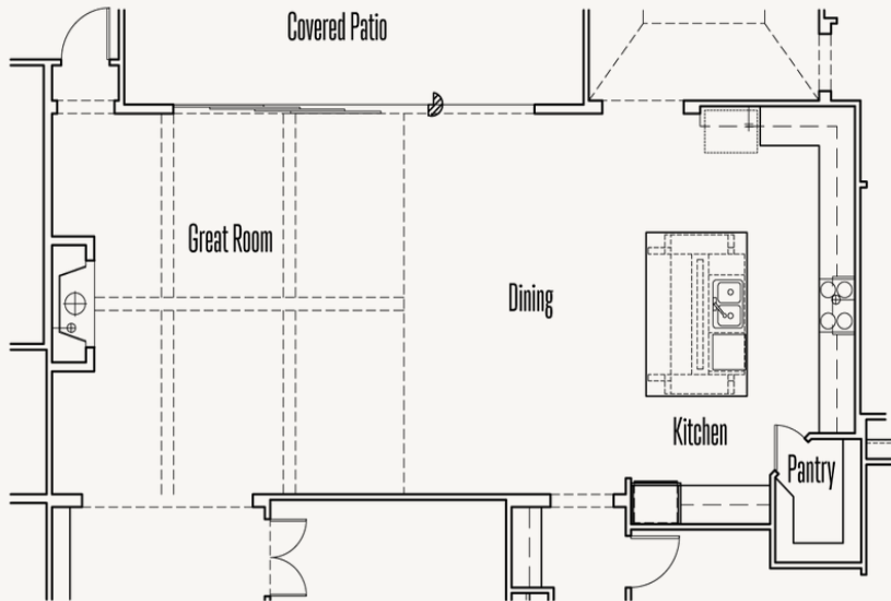
Optional Sliding Patio doors at Great Room
