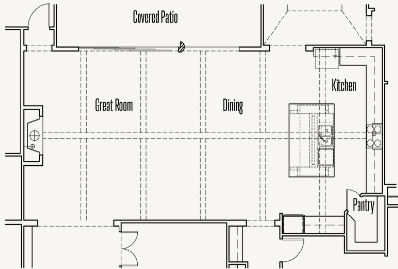
Optional Sliding Patio doors at Great Room w/ Cathedral Ceiling Treatment
