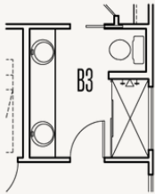
Optional Shower ilo tub in Bath #3
