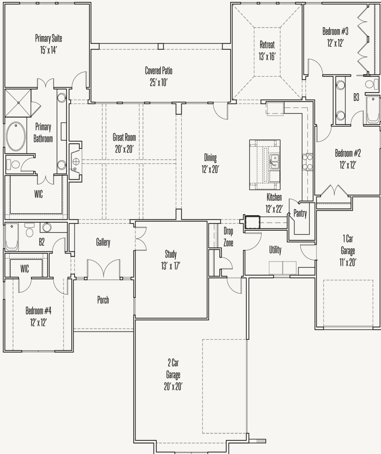
FLOOR PLAN_B
