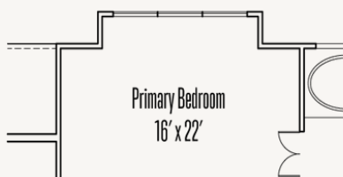
Optional Box Bay at Primary Bedroom
