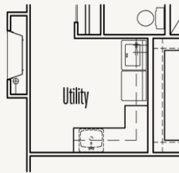
Optional Base & Full Upper Cabinets at Utility
