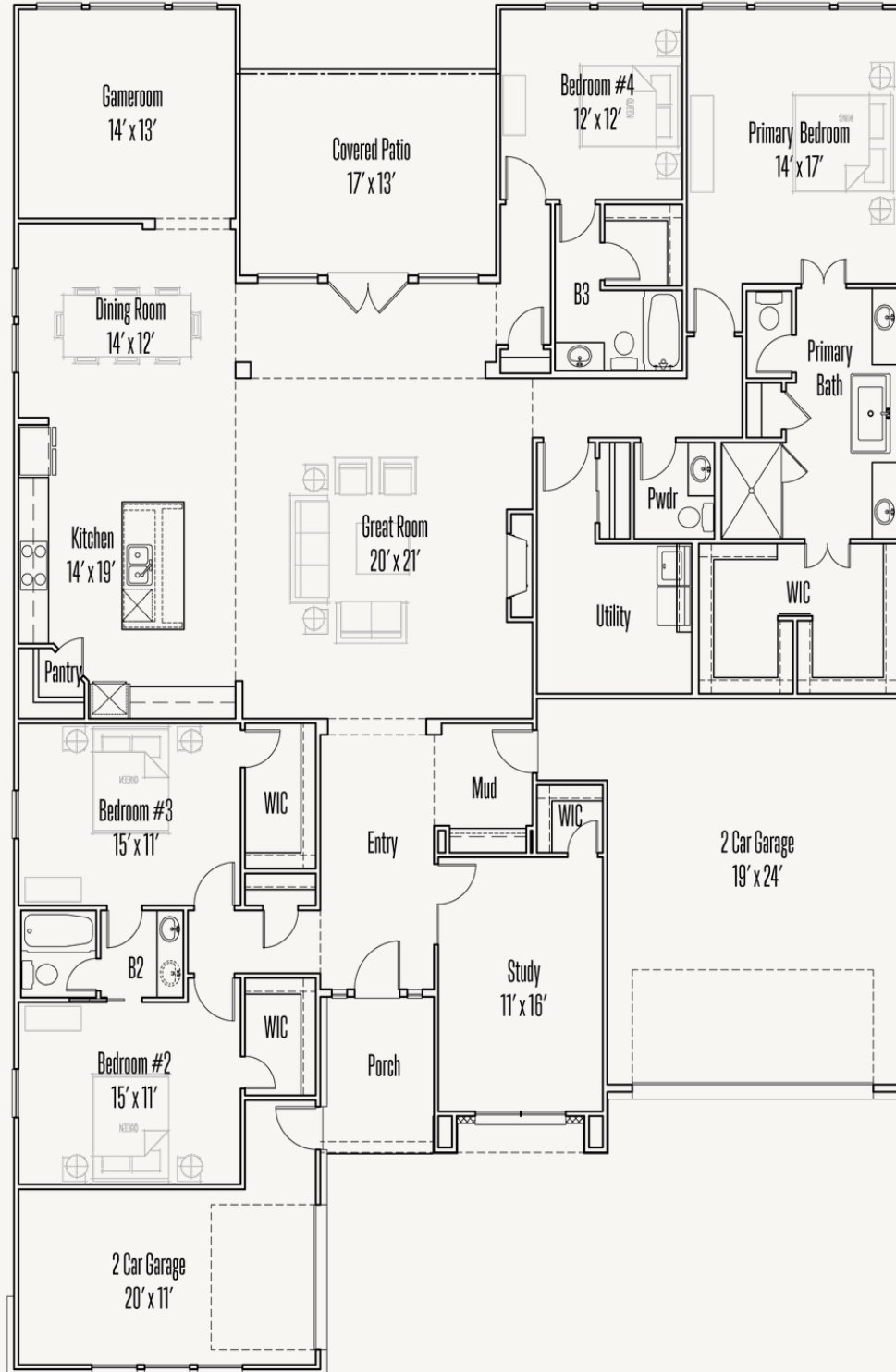
FLOOR PLAN_C
