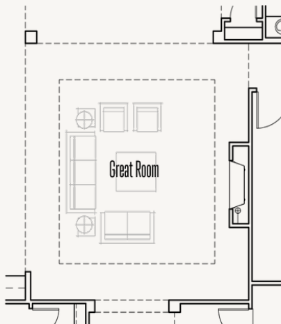
Optional Step Ceiling Treatment at Great Room
