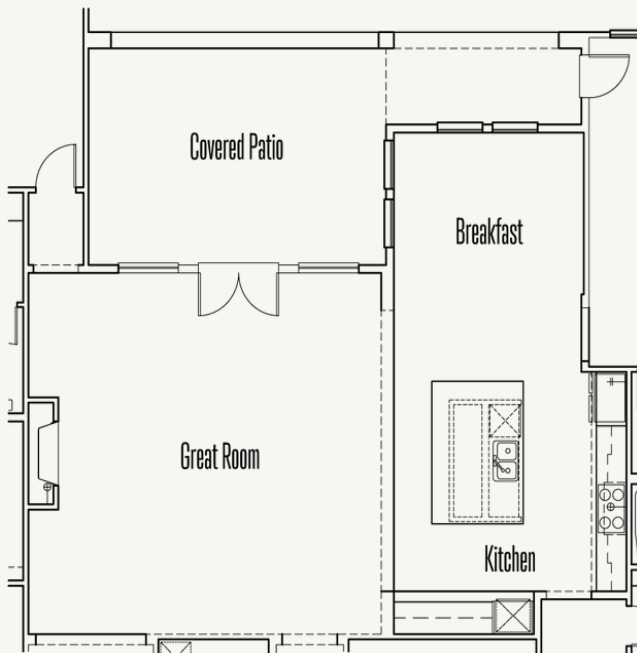
Optional 16' Ceiling at Great Room w/ 12' Ceiling at Kichen / Breakfast
